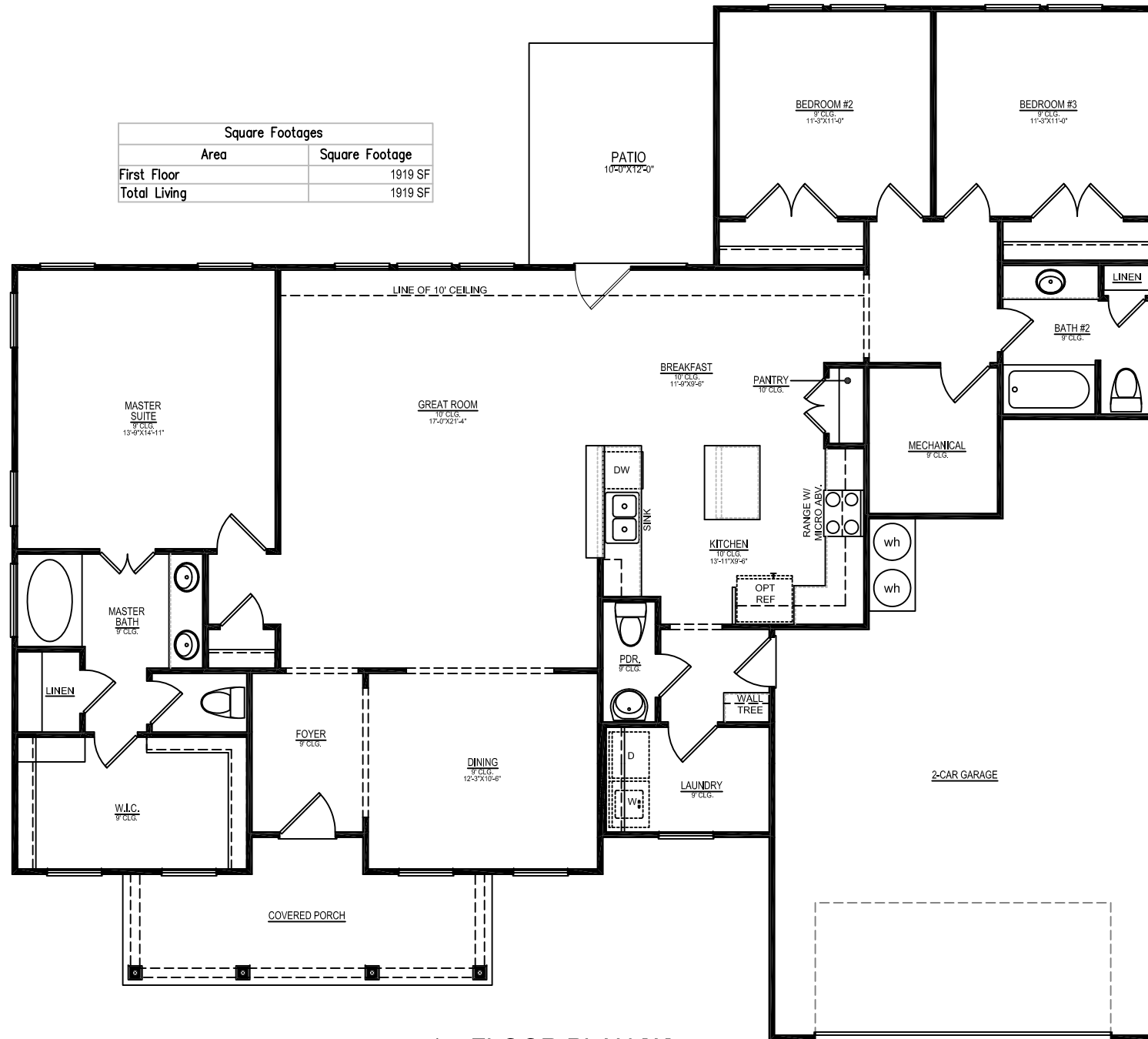
1st FLOOR PLAN [A]
